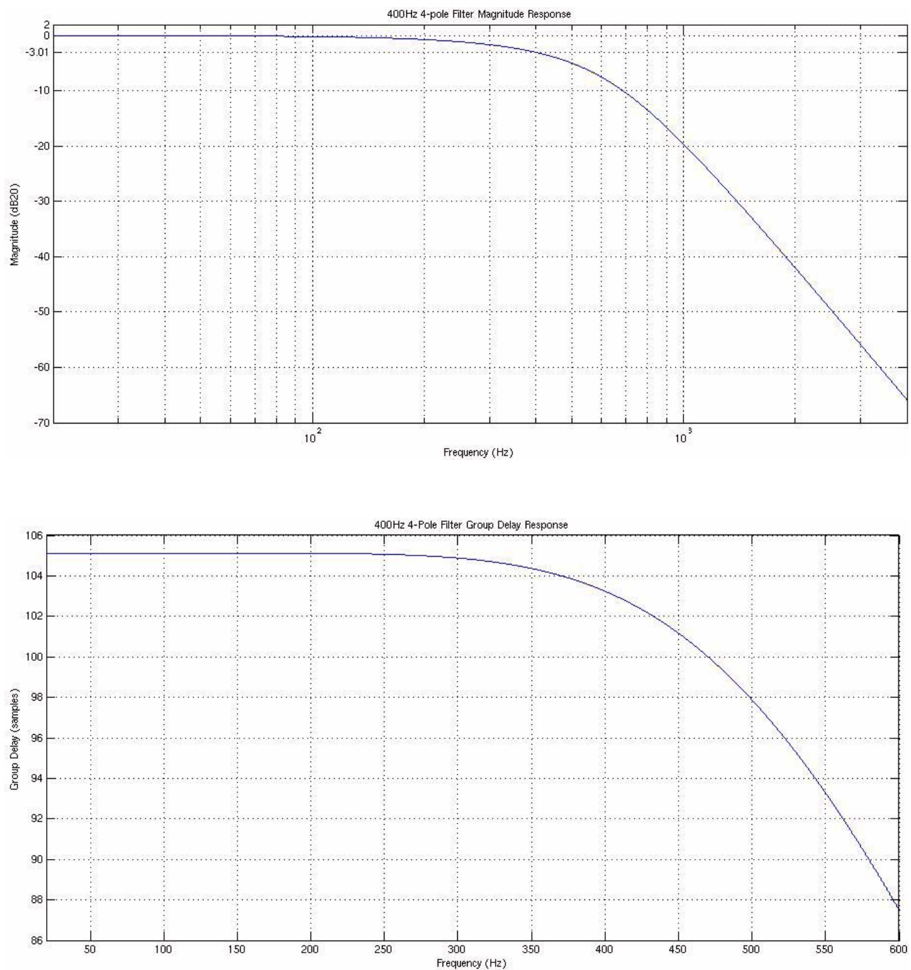
Figure 17. Low-Pass Filter Characteristics: f_C = 400\text{ Hz} , Poles = 4, t_S = 8\text{ }\mu\text{s}
